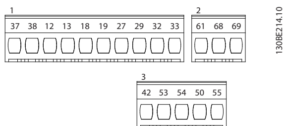
Illustration 2.9 Terminal Numbers
