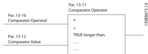
Illustration 2.36 Comparators
