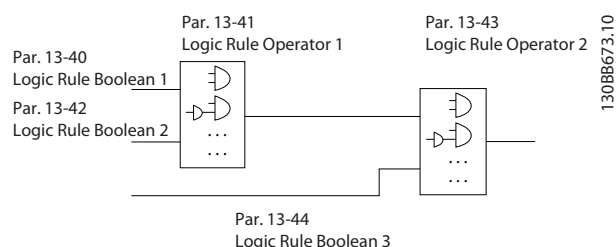
Illustration 2.37 Logic Rules
