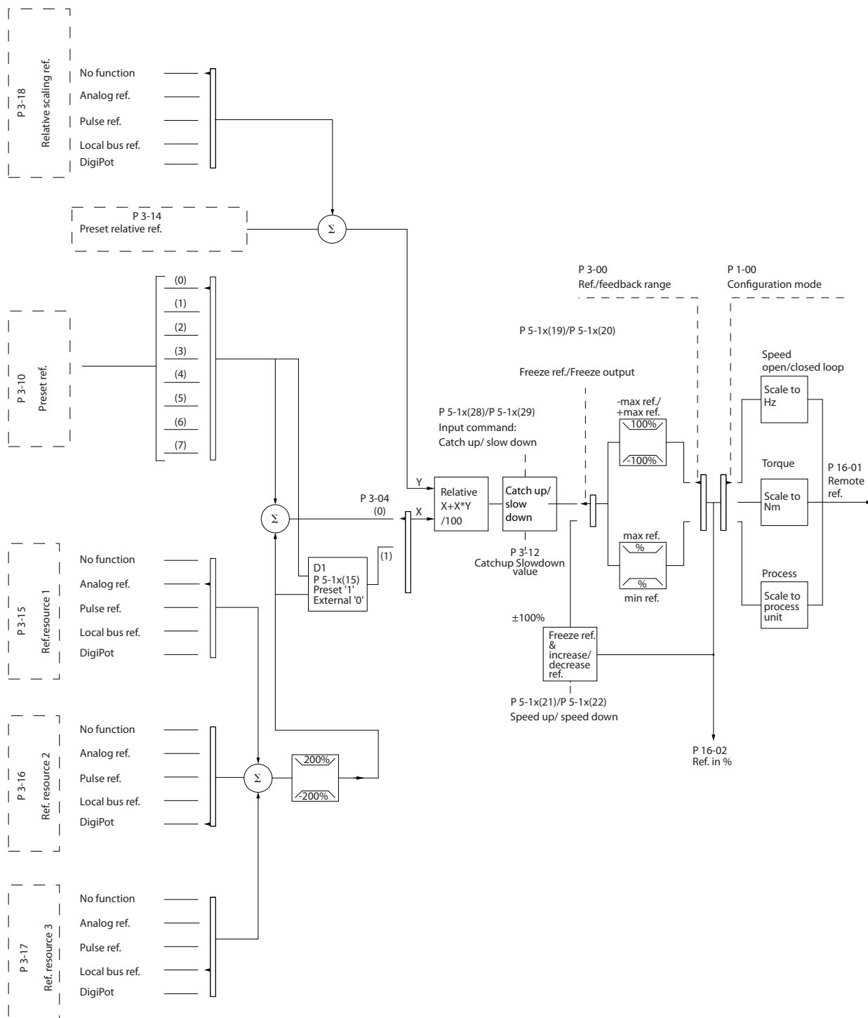
Illustration 2.14 Remote Reference
