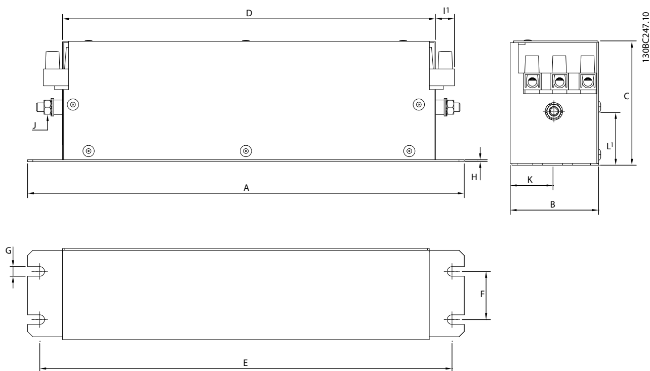
Illustration 6.3 Dimensions of EMC Filter for K4-K5
