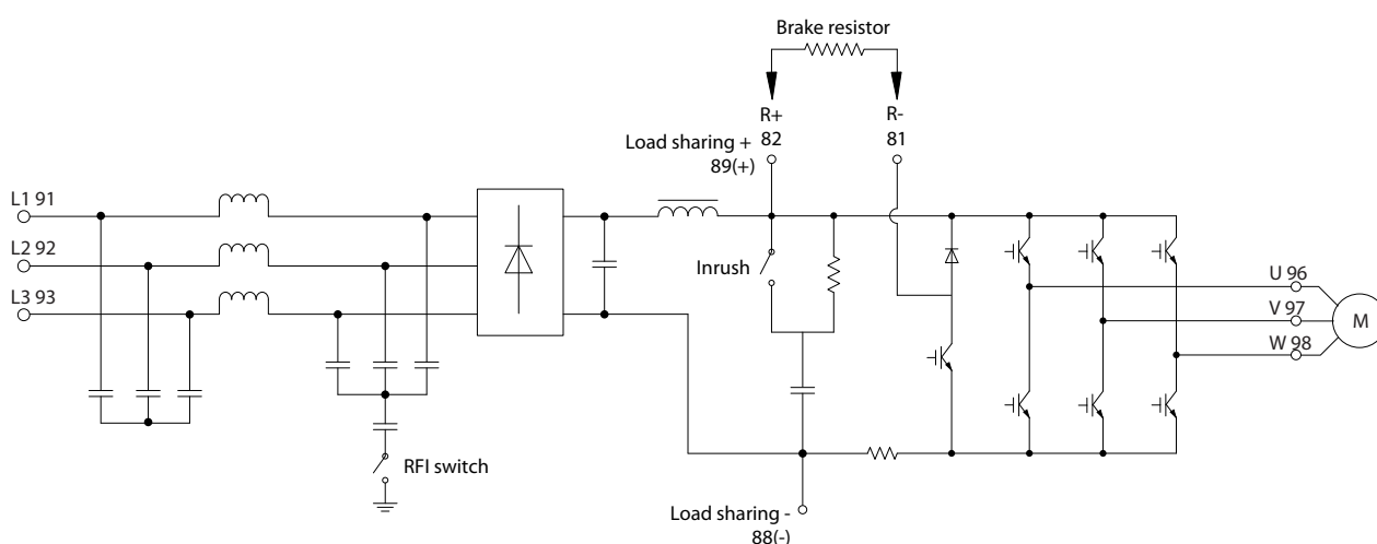
Illustration 2.10 Control Diagram
